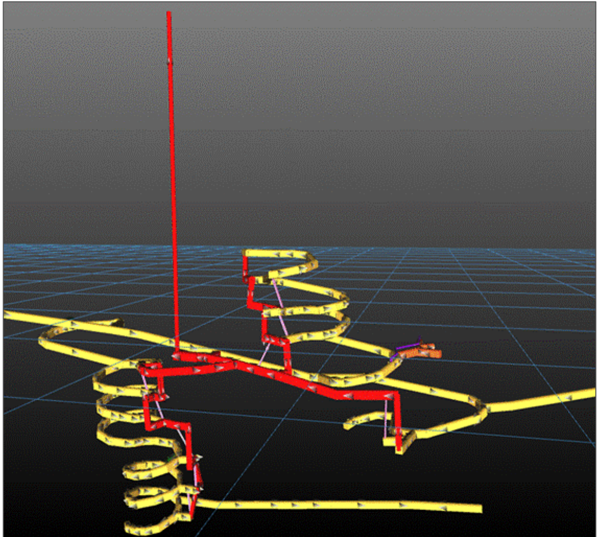
Figure 16.7: Cuffley primary ventilation circuit
