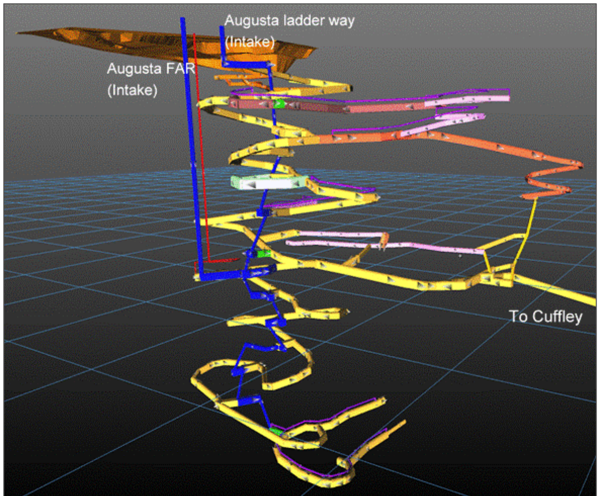
Figure 16.6: Augusta primary ventilation circuit
