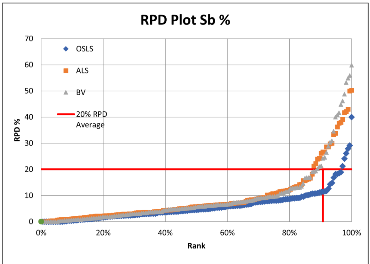
Figure 11.15: Relative paired difference plot, original versus umpire checks, for antimony analyses
