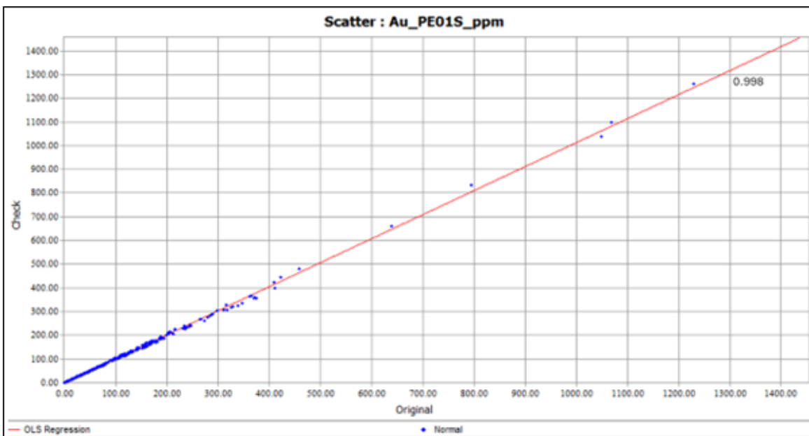
Figure 11.8: Scatter plot of On Site gold photon assay pulp duplicates (g/t)
