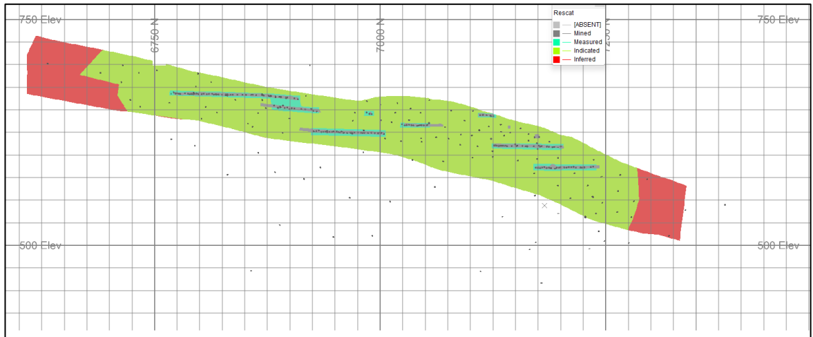
Figure 14.35: Suffolk 620 block model with resource category boundaries. lower intercepts not included were non-material below a bounding fault
