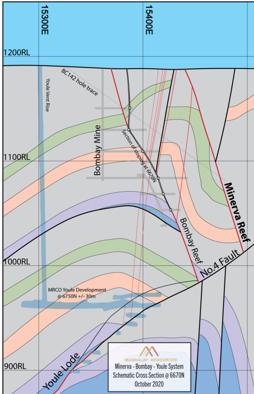
Figure 2: Section at 6670 northing illustrating the location and orientation of the new intercept on Minerva Reef.
